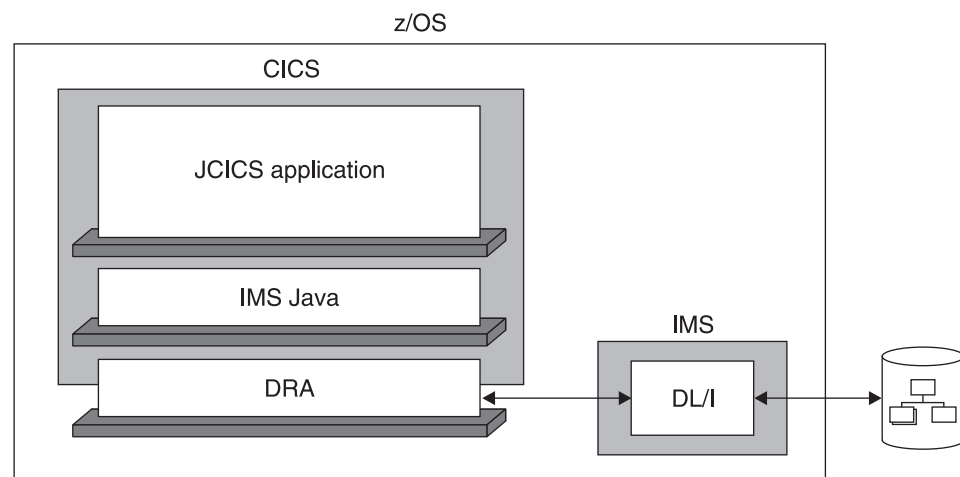
Figure 17. CICS Application Using IMS Java
